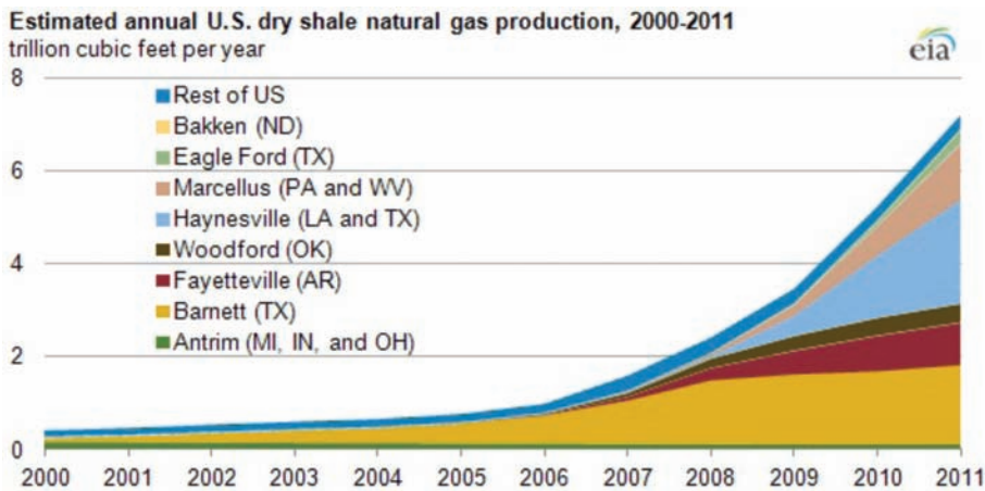
Figure 12: Evolution de la production de shale gas aux Etats-Unis (Source: EIA)
